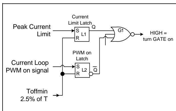
Figure 14 PWM Logic
