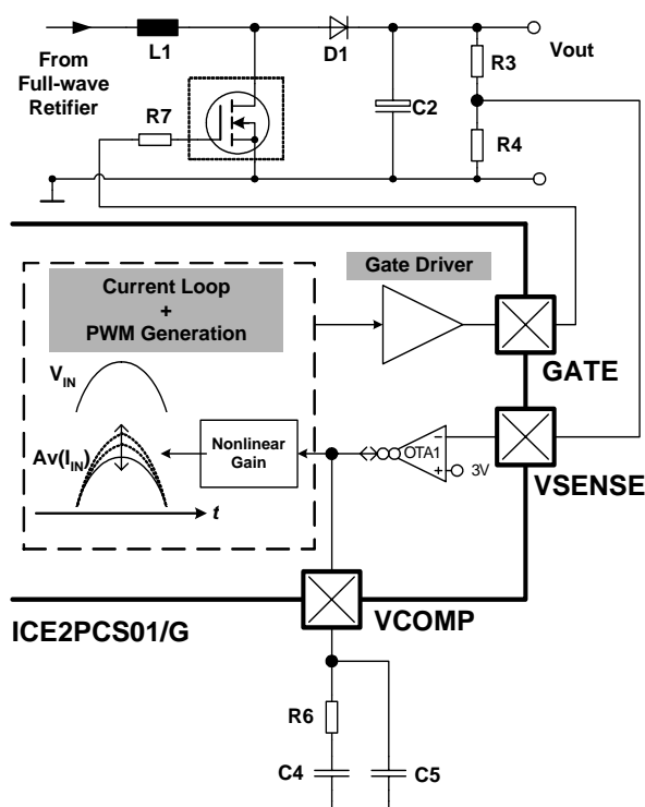
Figure 15 Voltage Loop
