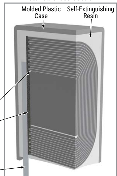
Detailed Cross Section
