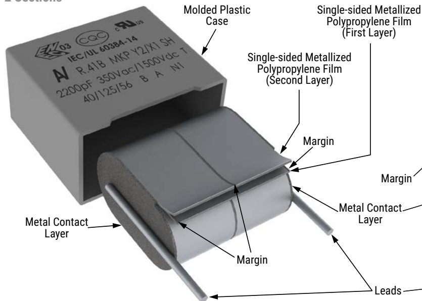
2 Sections
