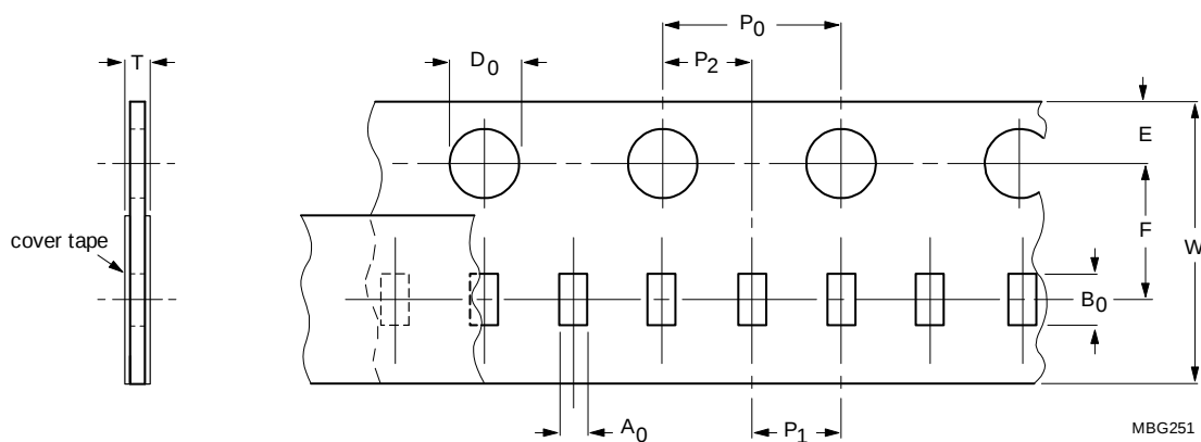
Fig. 15 Paper/PE Tape
