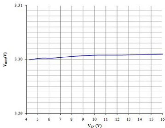
Figure 6: Line Regulation: I_{OUT} = 10\text{mA} , V_{OUT} = 3.3\text{V}
