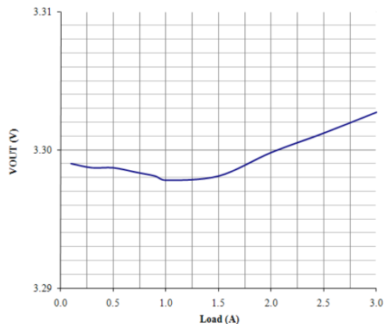
Figure 7: Load Regulation: V_{OUT} = 3.3\text{V}
