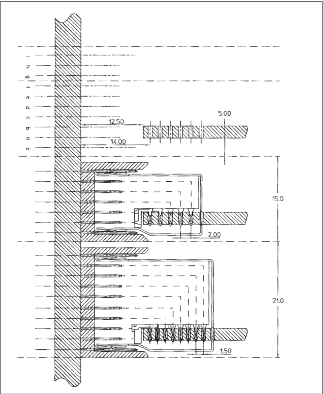
Built-in dimensions
