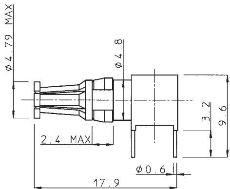
socket contact
