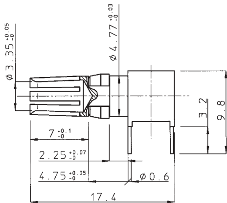
socket contact
