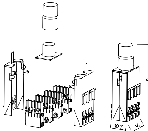
8 x 5 positions
