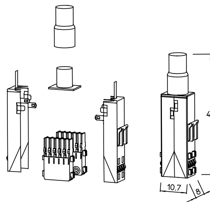
4 x 5 positions
