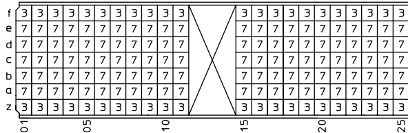
HM2P07PK5111GF
