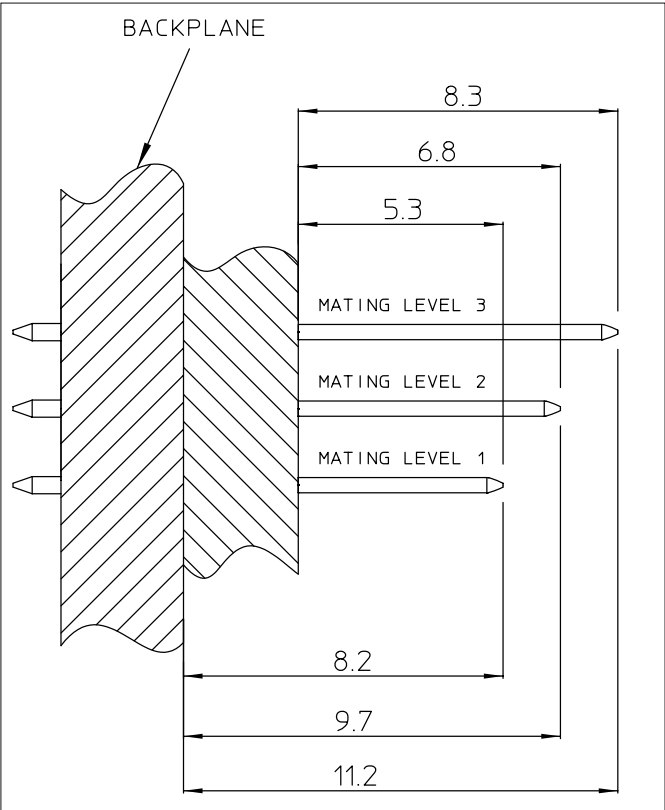
Signal contacts mating levels
