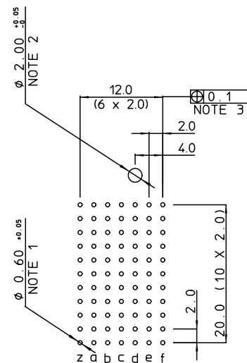
BACKPLANE LAY-OUT TYPE A,B,C AND CR
